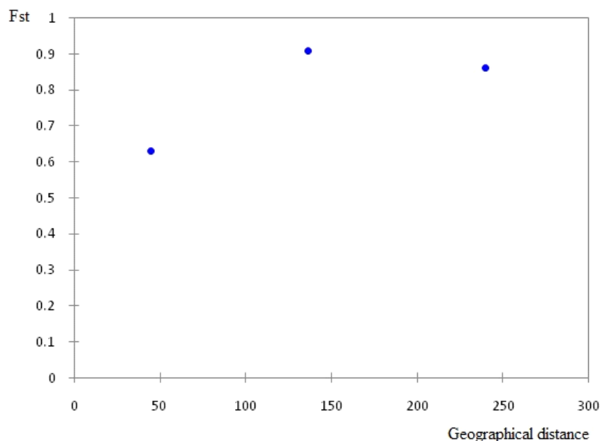
Figure 4. Correlation between geographical distance and genetic differentiation.
