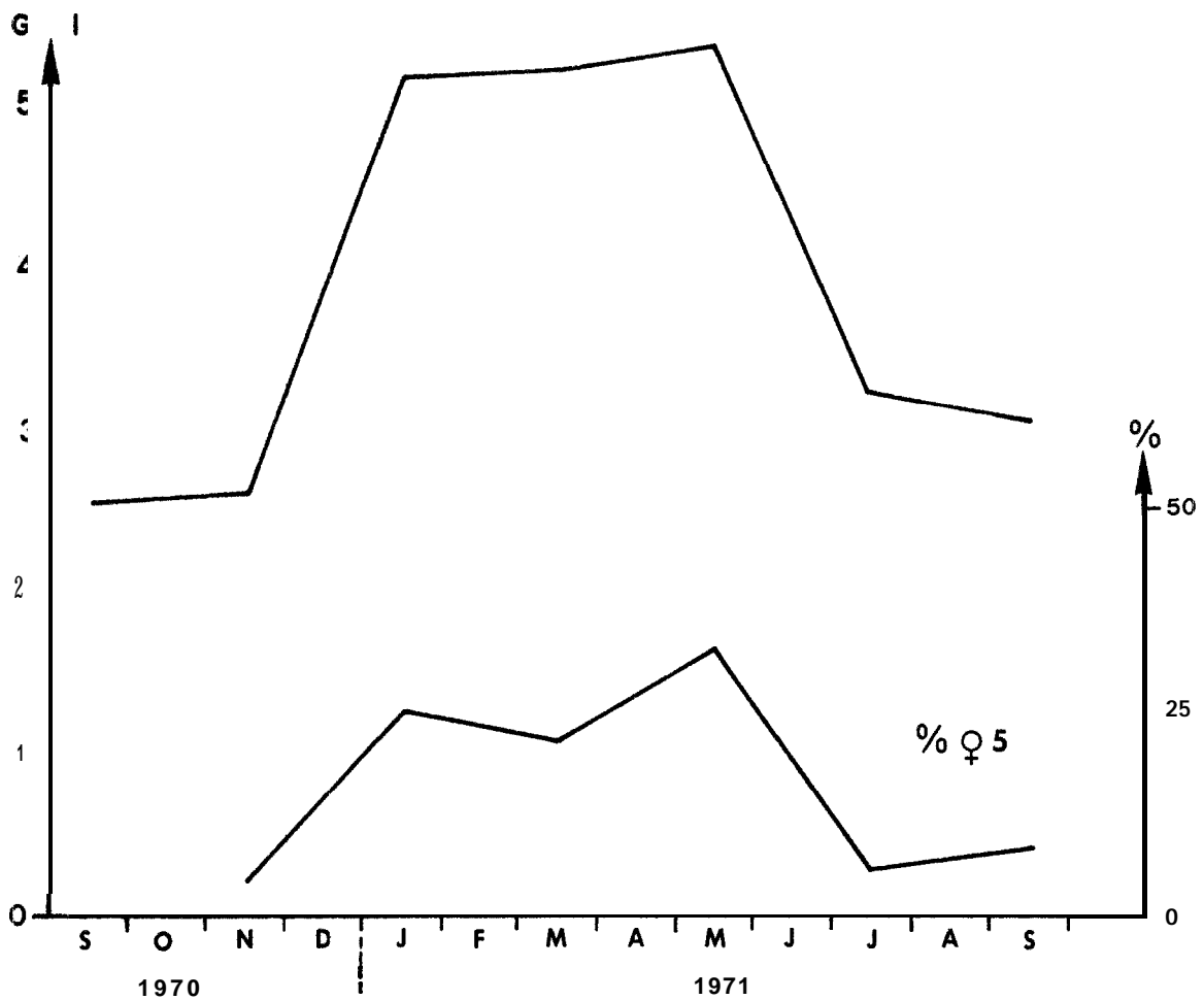
Fig. N°6 The bimonthly gonadosomatic index(G. S. I. ) of ethmalosa ( females) from the coastal area of The Gambia. The bimonthly percentages of females in maturity stage V.
