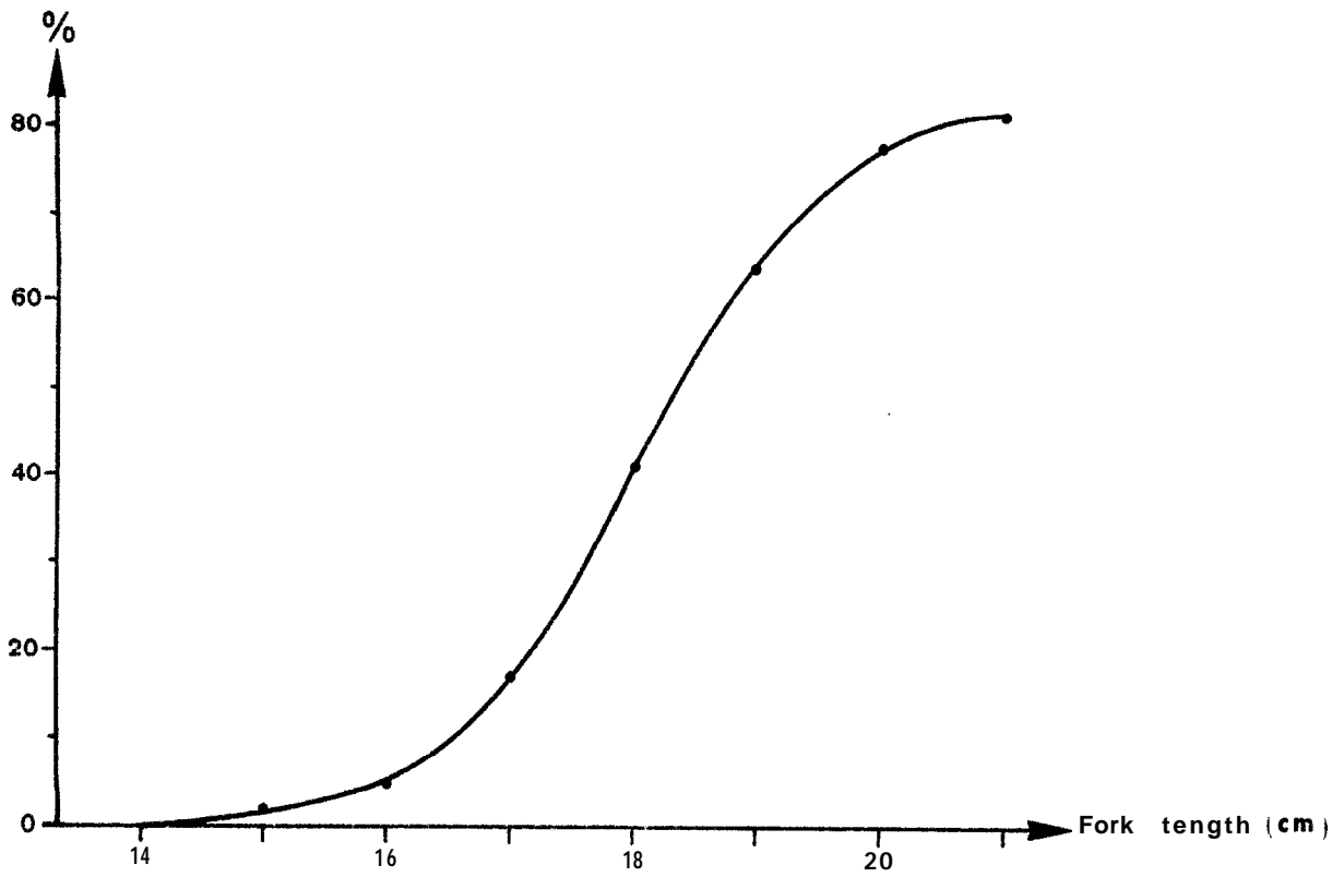
Fig. N°5 Percentages of grouped maturity stages ( stages IV ,V ,VI,VI-III ) of females in different length classes.
