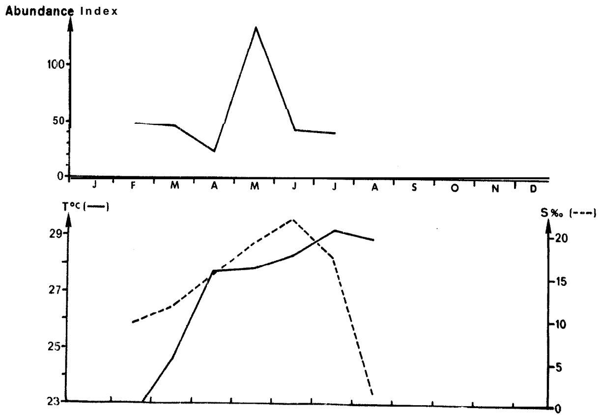
Fig. N°10 Monthly abundance of ethmalosa larvae and surface observations of temperature and salinity, in Balingho in 1974.
