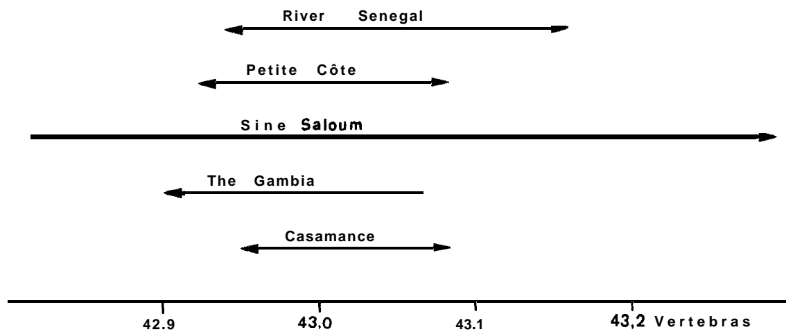
Fig. N°2 Average number of vertebrae and its confidence intervals ( 99% ) for different areas in the senegambian region.
