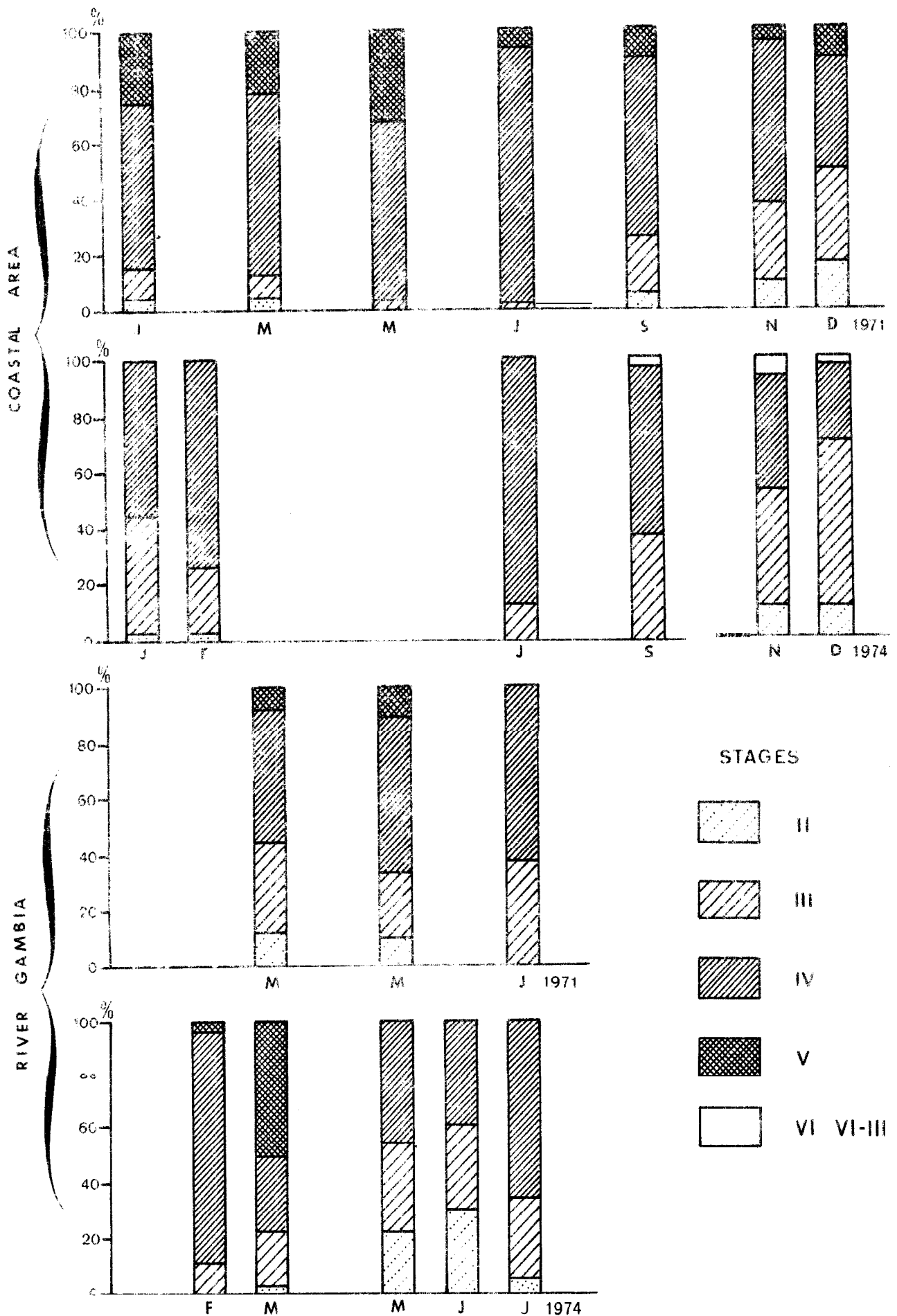
Fig. N°7 Monthly percentages of different maturity stages of Ethrnalosa fimbriata from samples of the coastal area and the river Gambia .
