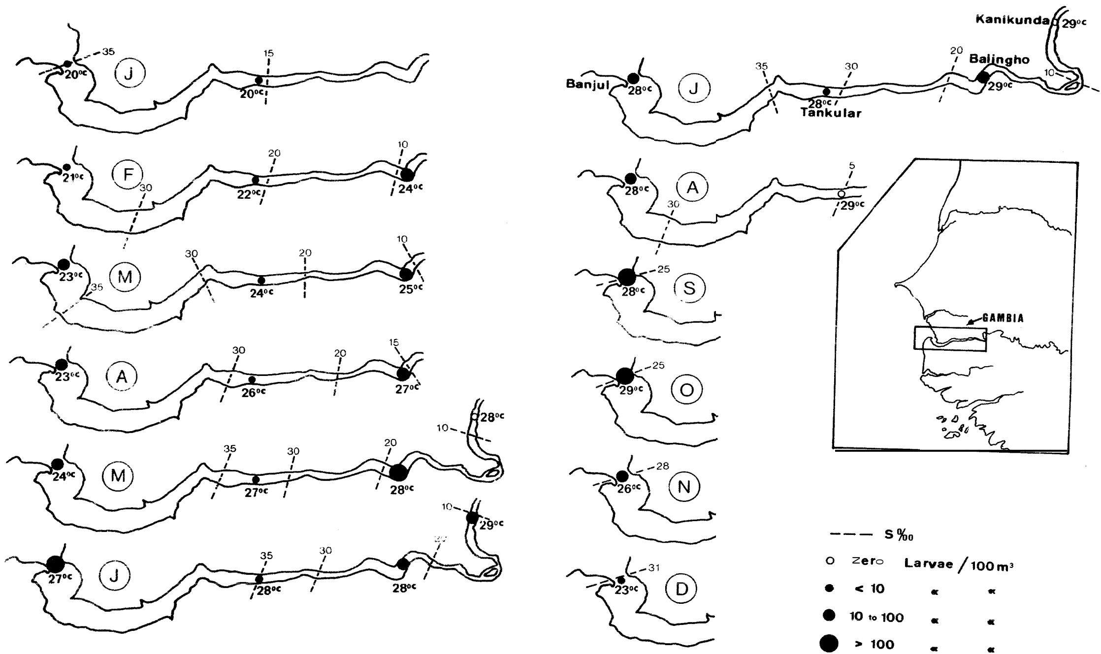
Fig. N°8 Abundance of Ethmalosa fimbriata larvae in the Gambia during 1974.
