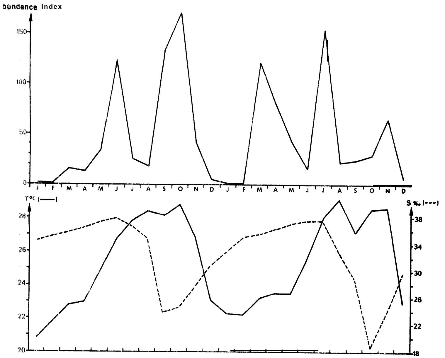
Fig. N°9 Monthly abundance of ethmalosa larvae, and surface observations of temperature and salinity, in Banjul in 1974 and 1975
