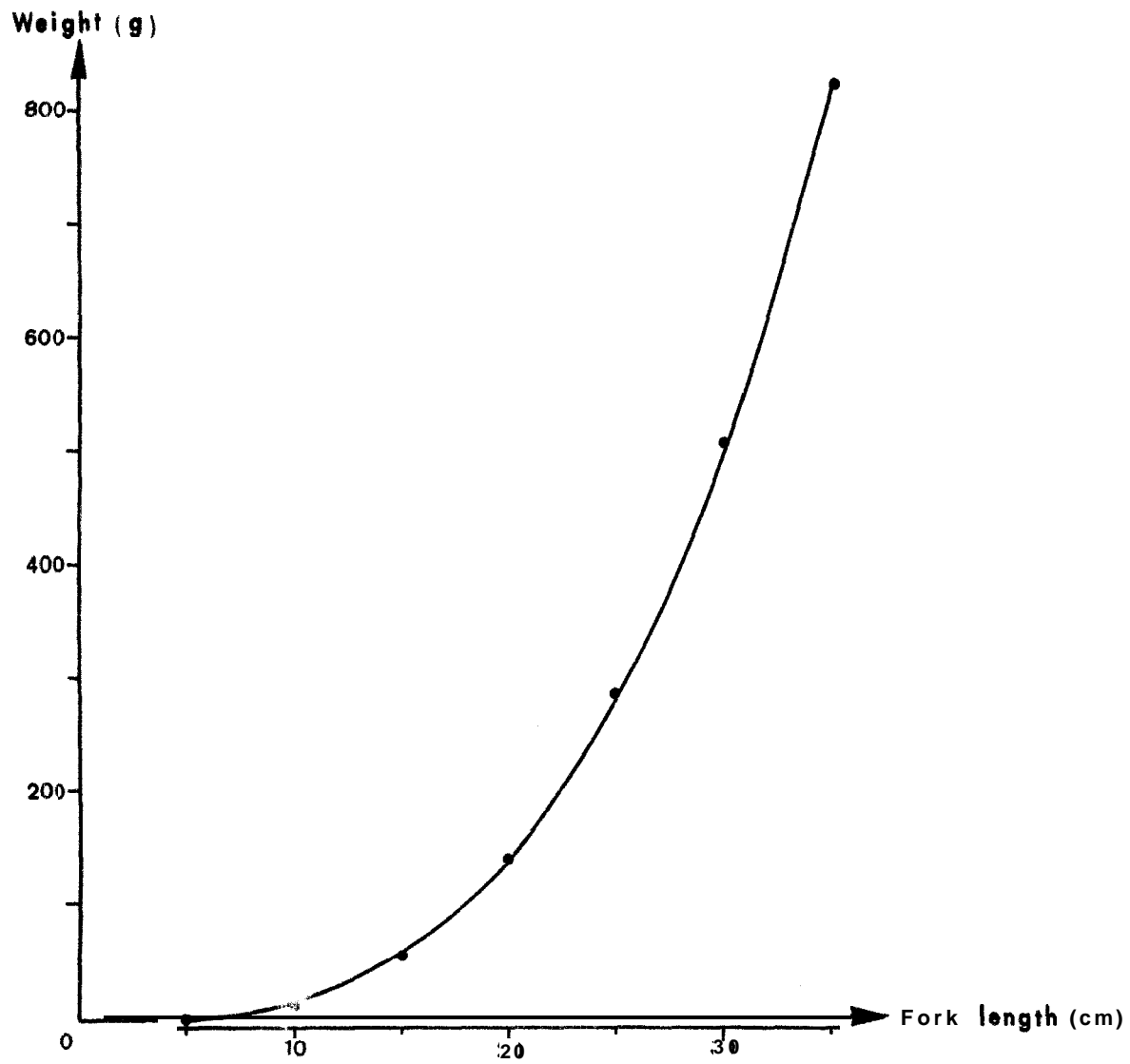
Fig. N°1 Length-weight relationship for Ethmalosa fimbriata from gambian waters.
